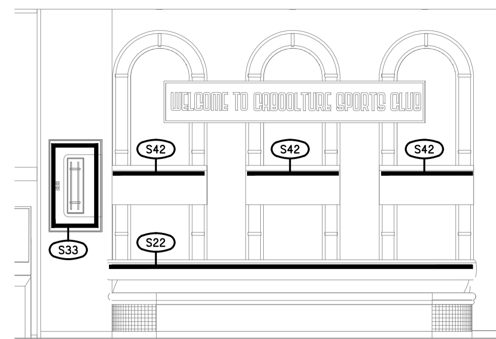
DETAIL A2 ENTRY S22 & S40 ELEVATION SCALE 1:50
