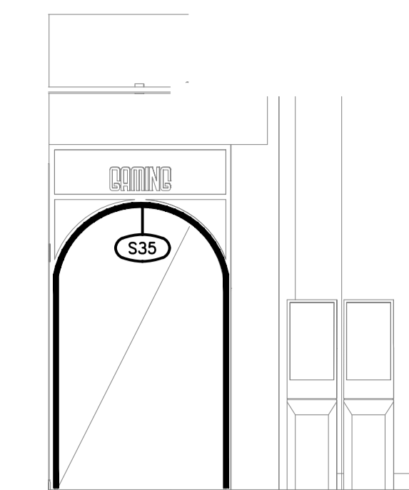
DETAIL A1 ENTRY S35 ELEVATION SCALE 1:50
