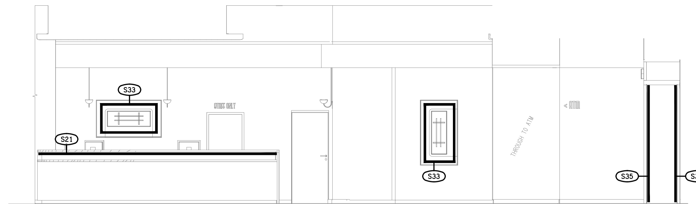
DETAIL A3 RECEPTION S21 & S35 ELEVATION SCALE 1:50
